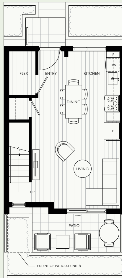
MAIN LEVEL
